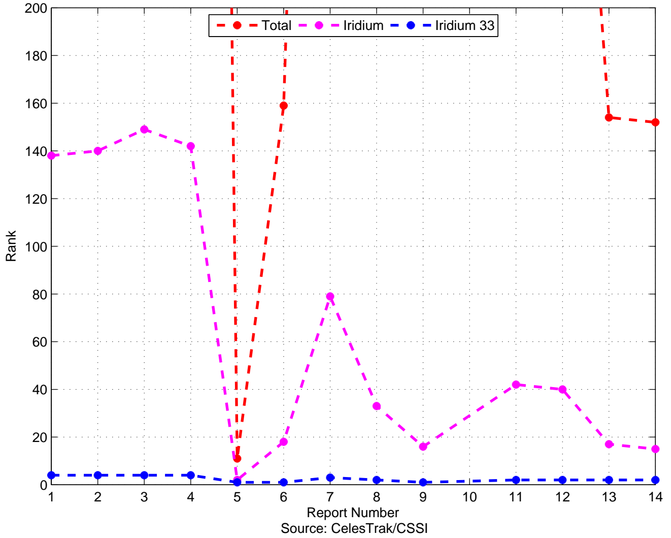
SOCRATES Rank
