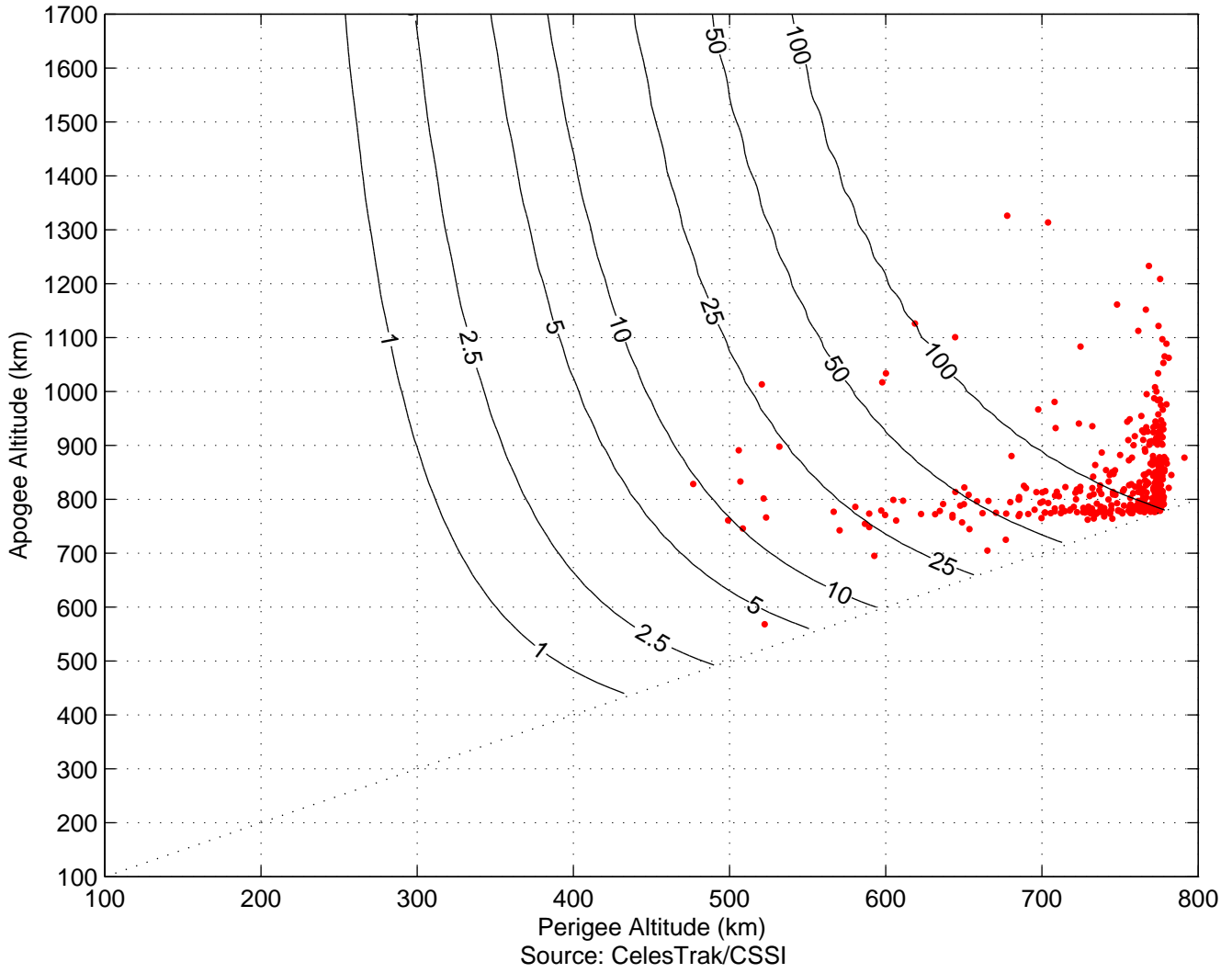
Apogee-Perigee Lifetime Plot of Iridium 33 Debris (398 pieces, average radius)
