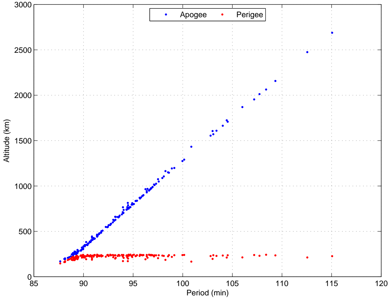
Gabbard Plot of USA 193 (2006–057) Debris (173 pieces)
