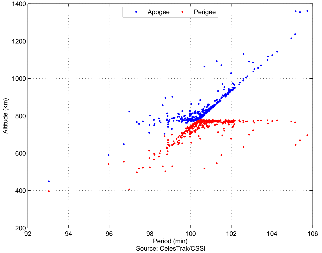
Gabbard Plot of Iridium 33 Debris (351 pieces)
