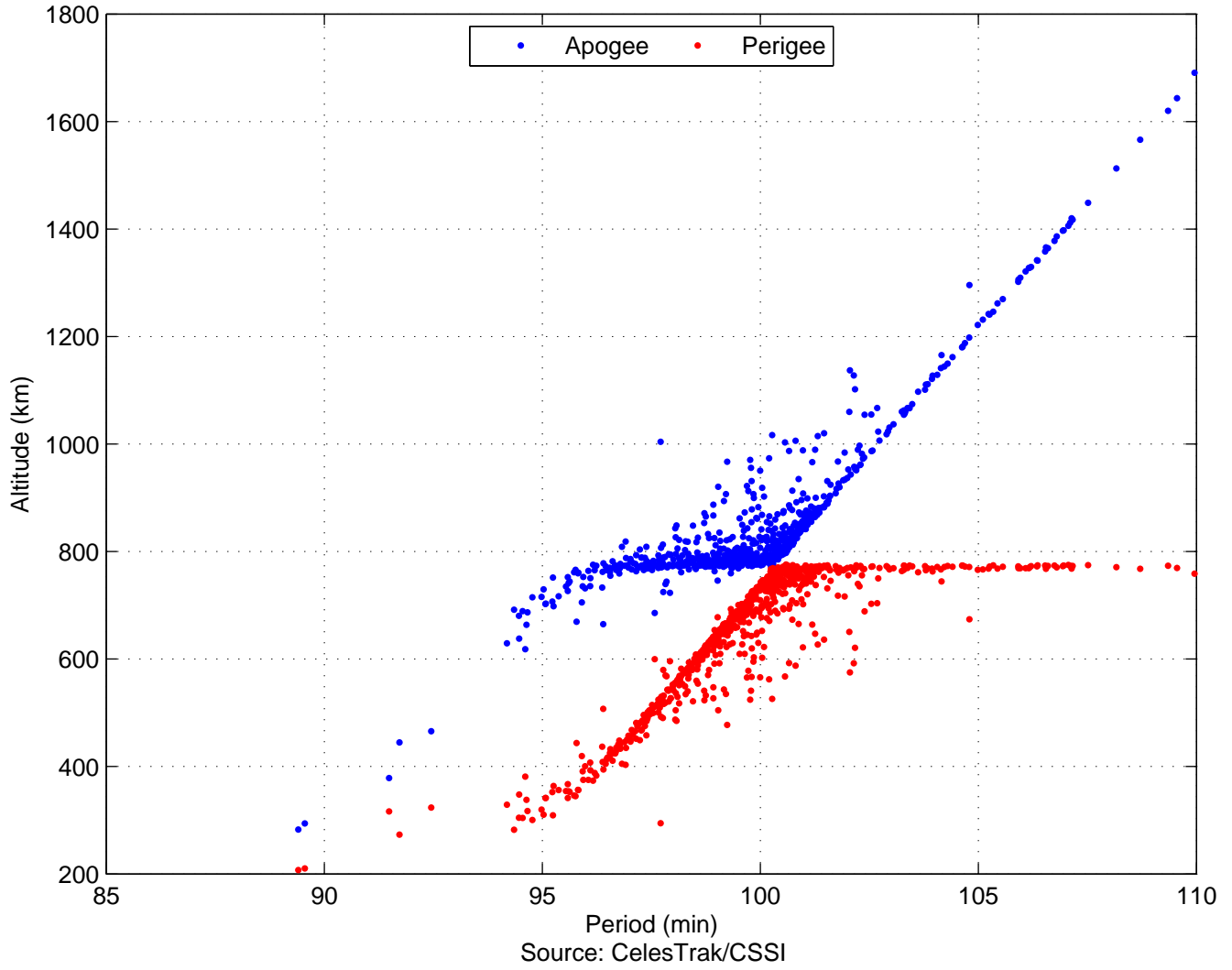
Gabbard Plot of Cosmos 2251 Debris (825 pieces)
